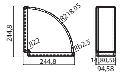
KOLJENO CRO 90 220X90 MM FUN 112.0459.455
