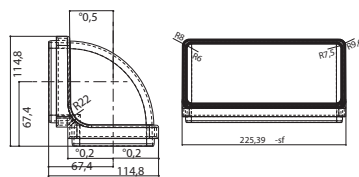
KOLJENO CRV 90 220X90 MM FUN 112.0459.453
